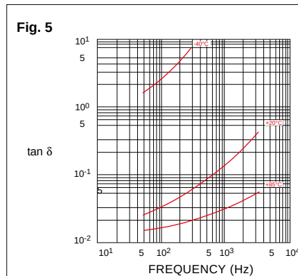
\tan \delta DRIFT VERSUS FREQUENCY HIGH VOLTAGE ( > 100\text{ V}_r d.c.)
